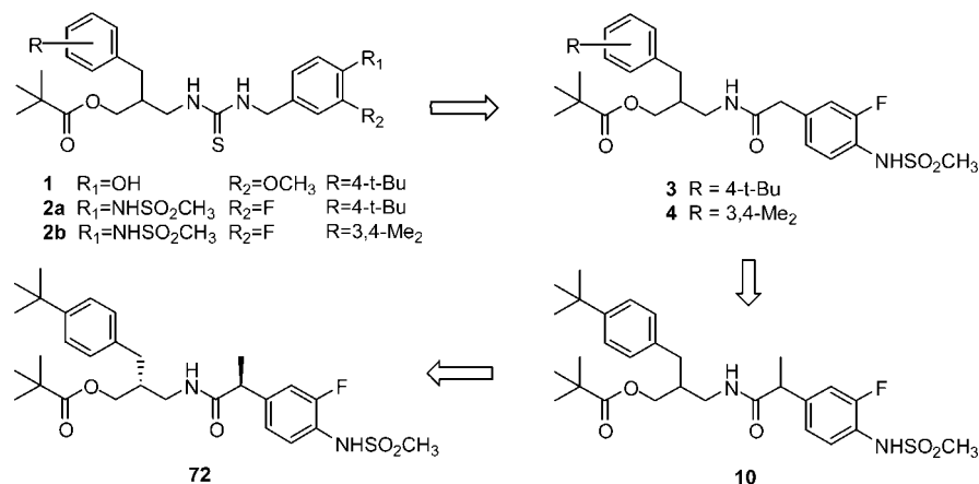
Scheme 1. Synthesis of Racemic and Diastereomeric Analogues a
