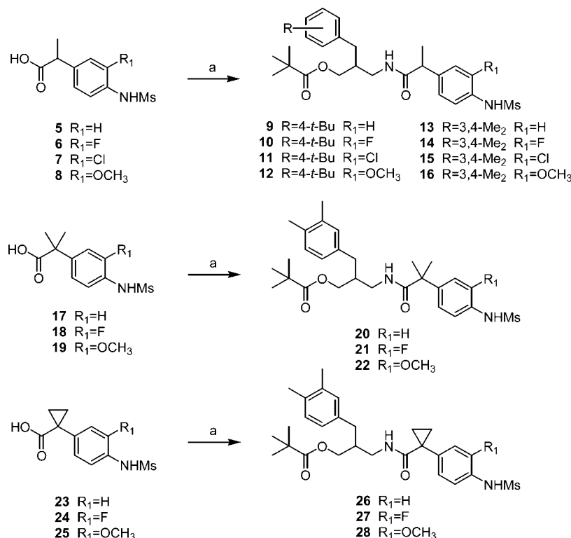
Scheme 1. Synthesis of Racemic and Diastereomeric Analogues a
